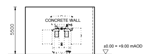
ELEVATION NORTHEAST
