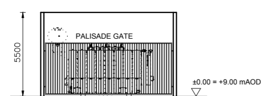
ELEVATION SOUTHEAST
