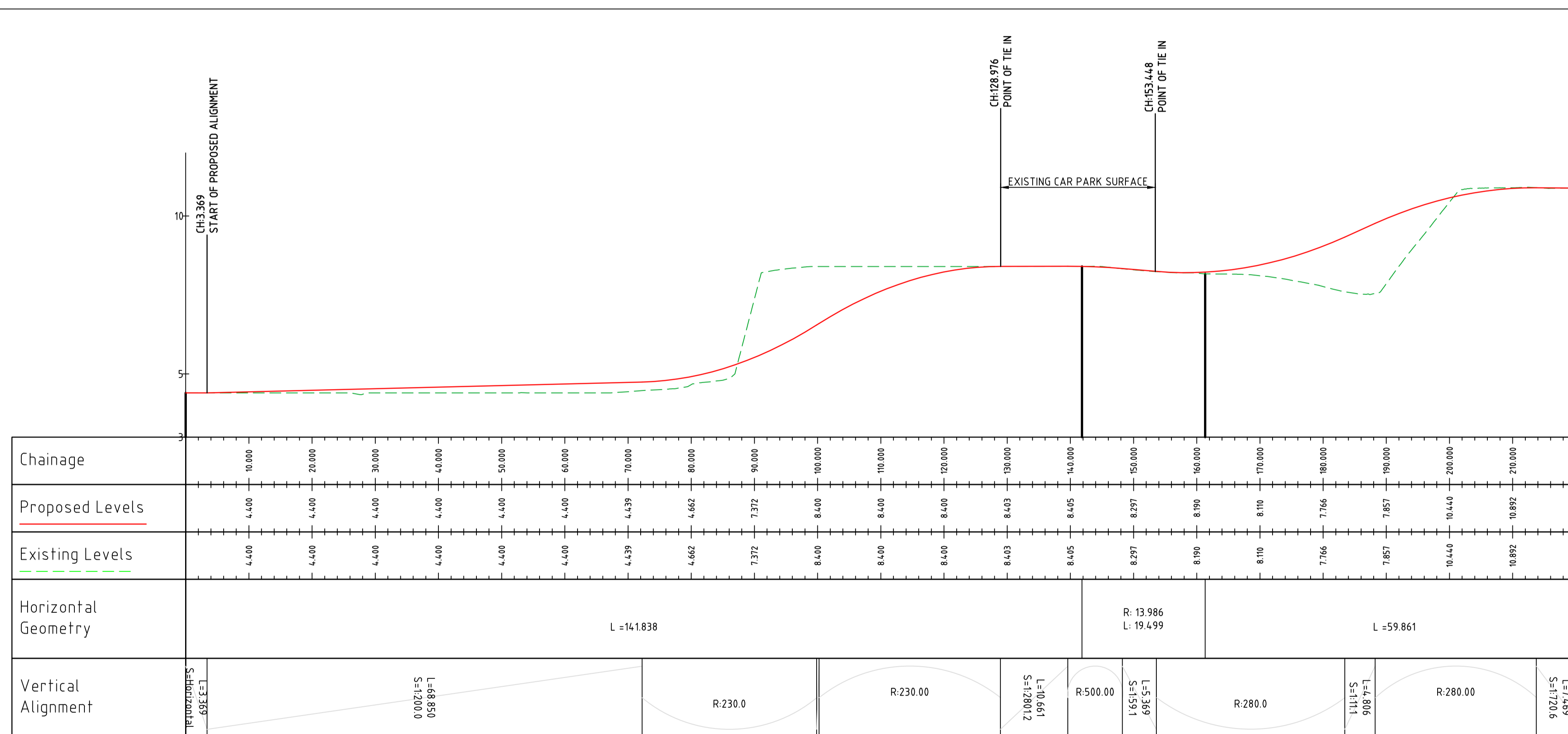
BULLPOINT LONGSECTION SCALE: H 1:500, V 1:100
